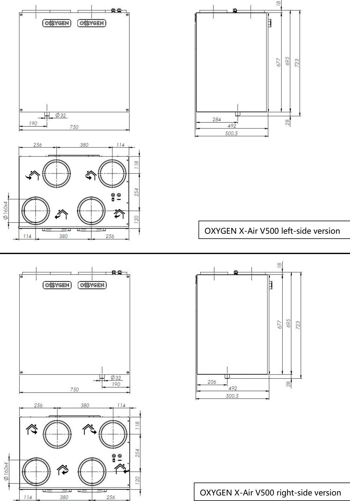
Figure 1. Unit dimensions
