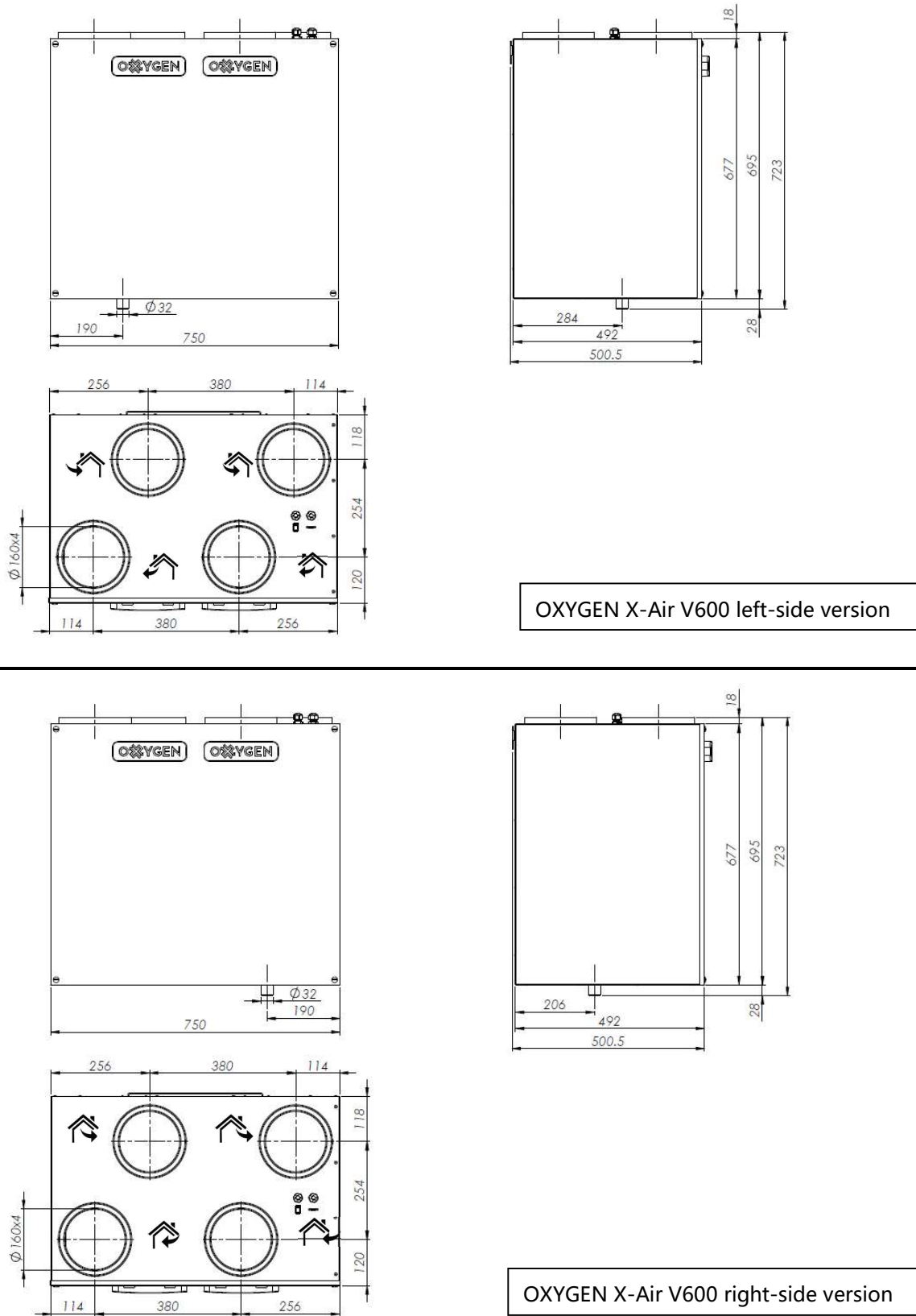
Figure 1. Unit dimensions
