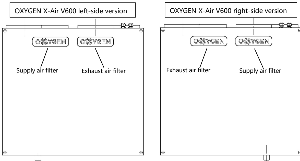
Figure 28. Locating air filters
